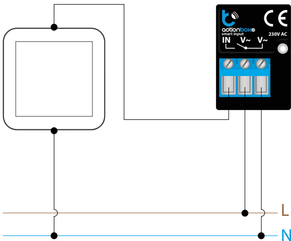
Connection diagram (case 1):
